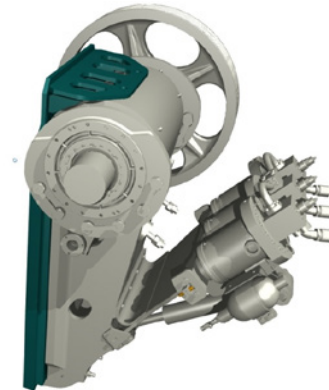
Active Setting Control (ASC) for C96, C106, C117, C120, C130 and C150 to enhance performance & protect the crusher in hard applications with frequent uncrushable objects.
